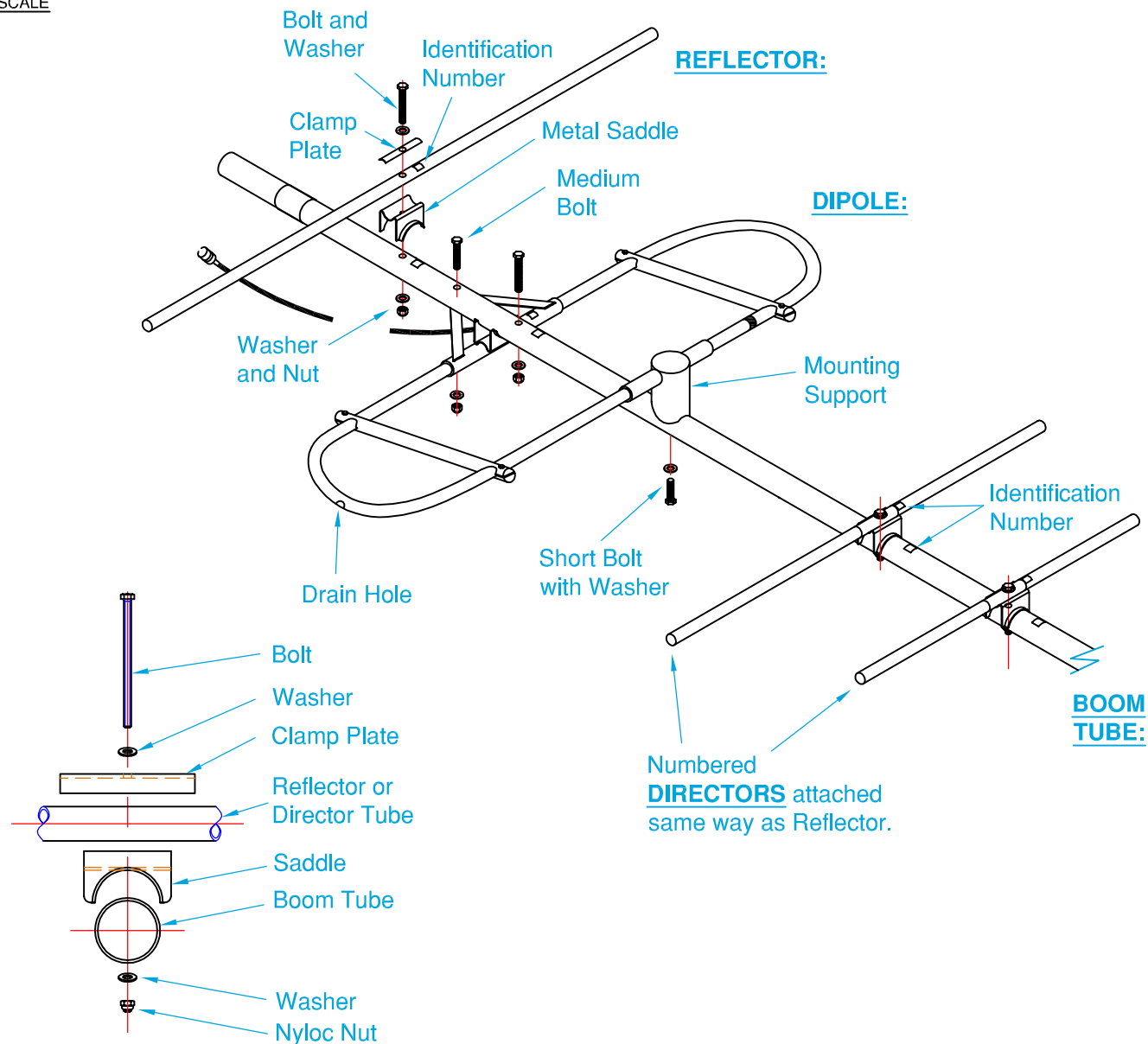
Typical Saddle Assembly
