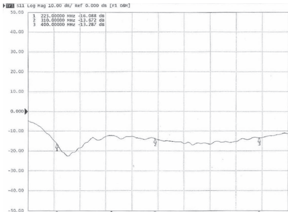
Typical VSWR
