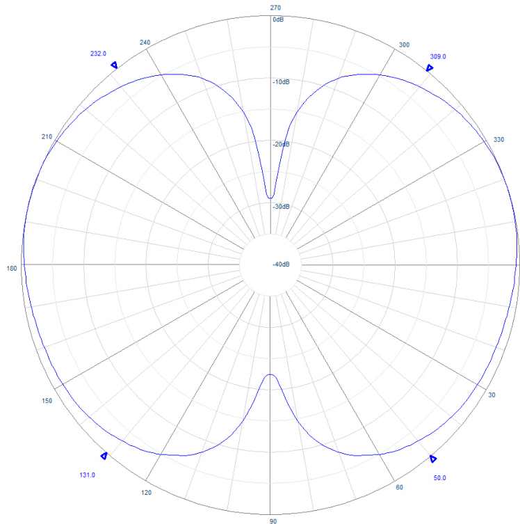
Example radiation pattern at 310 MHz
