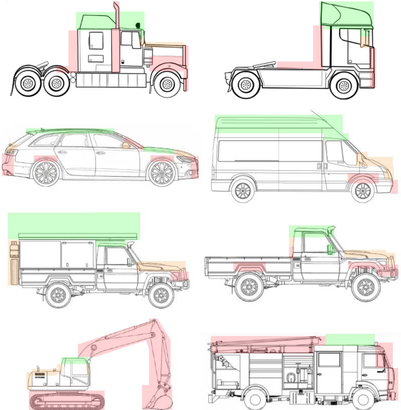
Recommended vehicle mounting locations
